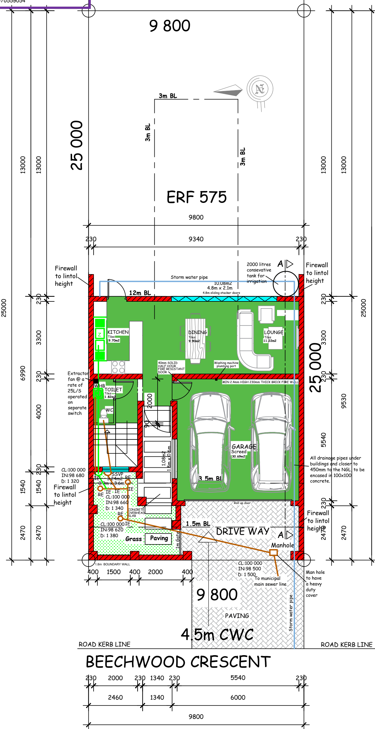
GROUND STOREY PLAN SCALE 1:100 83.94m 2
