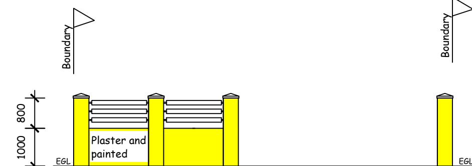
WEST BOUNDARY ELEVATION SCALE 1:100
