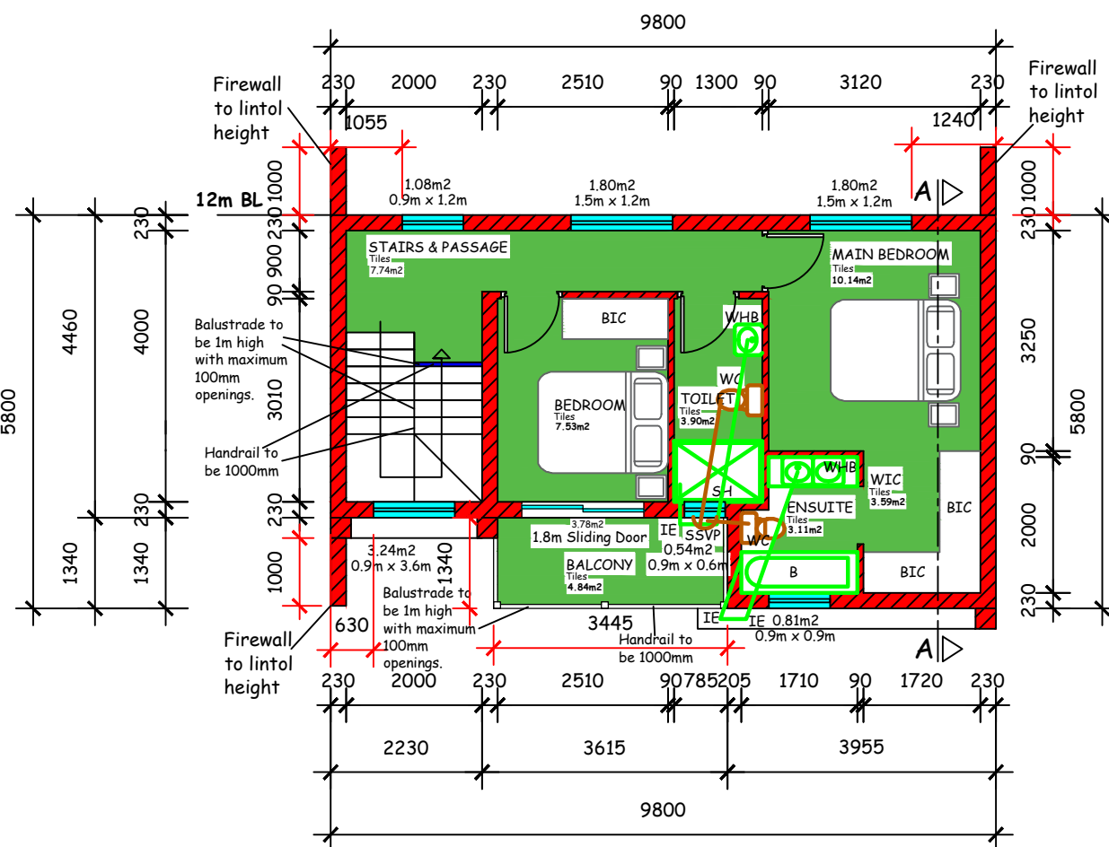
FIRST STOREY PLAN SCALE 1:100 46.77m 2
