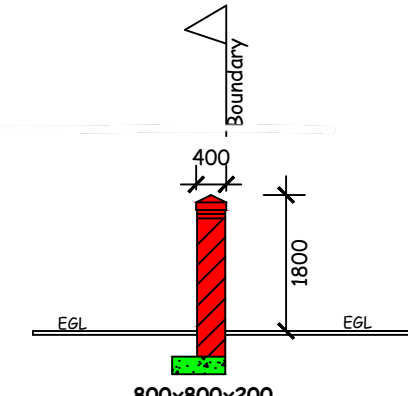
SECTION THROUGH PILLAR SCALE 1:100
