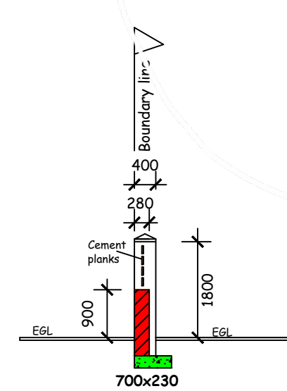
SECTION THROUGH BOUNDARY WALL SCALE 1:100
