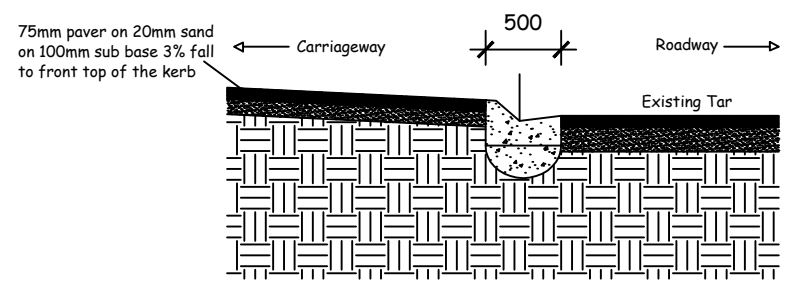
KERB SECTION DETAIL SCALE 1:50
